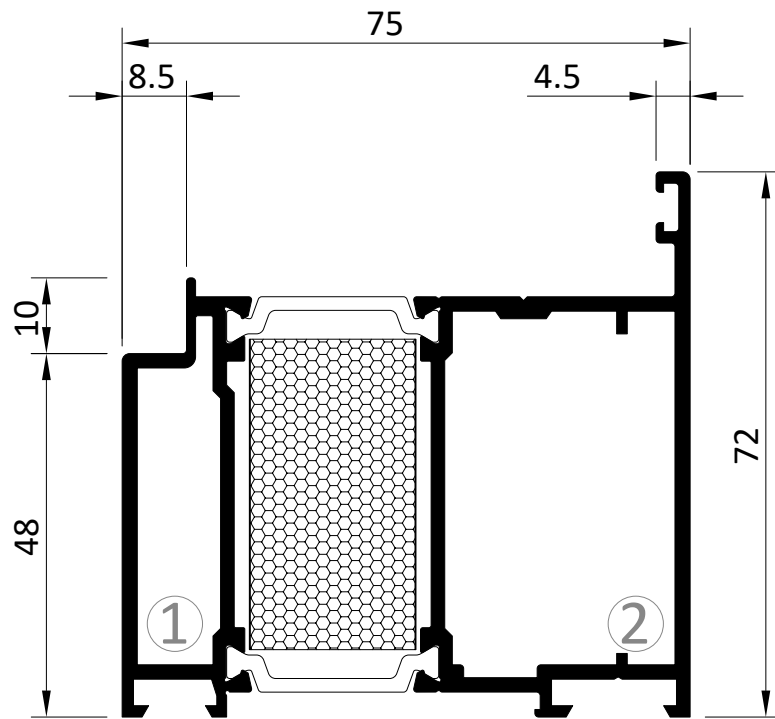
1426 Rahmen Frame Isolator Insulation 2213
