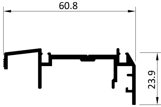
2754 Pendelstulp Double action
