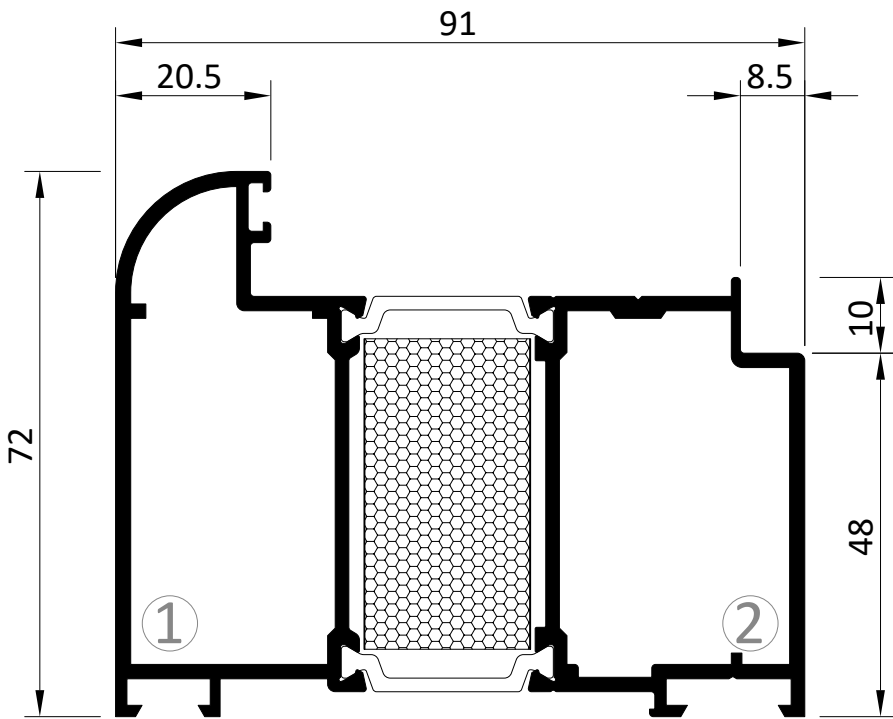
1422 Softline Softline Isolator Insulation 2213
