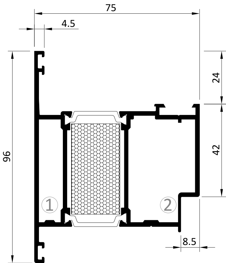
1432 Flügel Leaf Isolator Insulation 2213
