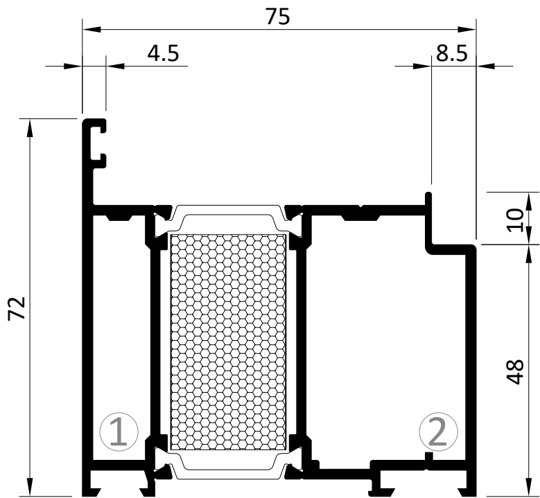
1425/1415 Rahmen Frame Isolator Insulation 2213
